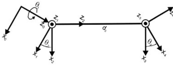
Figure 10. D-H frames for a spatial curve.
