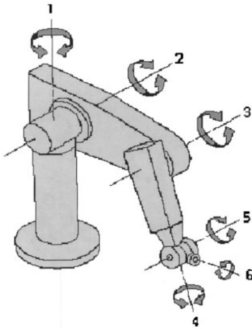
Figure 1. Discrete manipulator.
