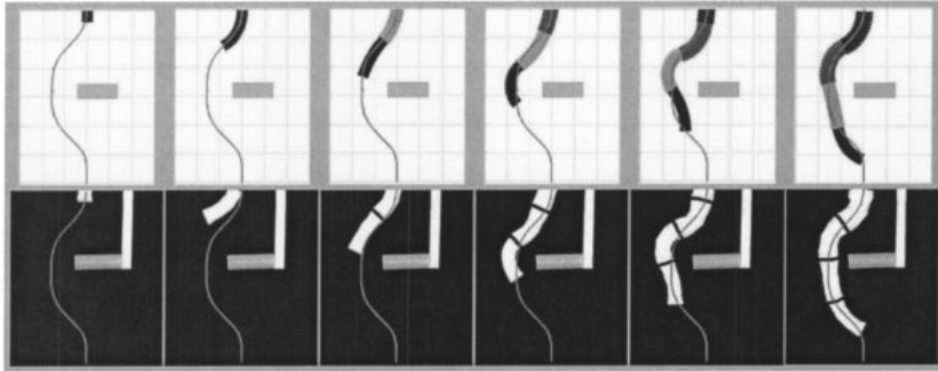
Figure 19. Obstacle avoidance using a static curve (top row is simulation, bottom column is experiment).
