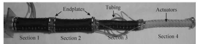
Fig. 5. Octarm IV continuum manipulator
